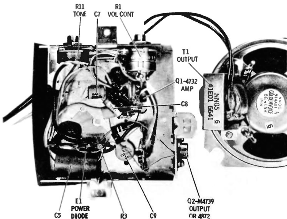
PARTS LOCATION
